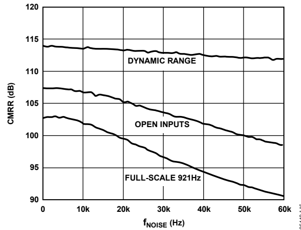
Figure 22. AD7766 CMRR vs. Common-Mode Ripple Frequency ( f_{NOISE} )
