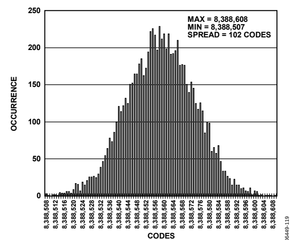
Figure 24. AD7766-1 24-Bit Histogram
