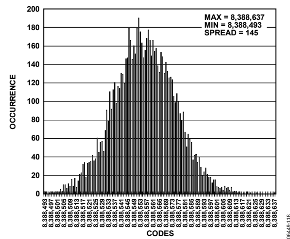
Figure 23. AD7766 24-Bit Histogram
